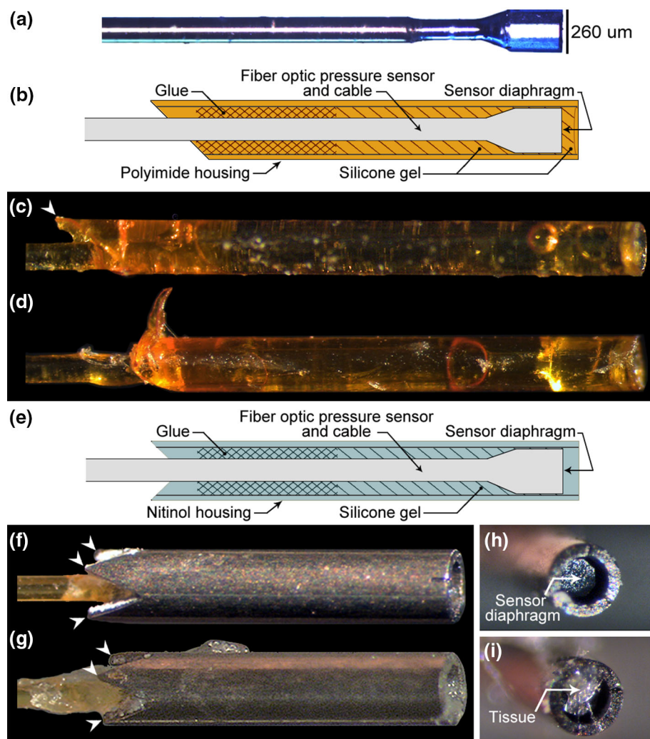
FIGURE 1. (a) A representative image of a pressure microsensor with no housing. (b) Detailed assembly drawing of the polyimide housing sensor. A barbed polyimide housing sensor (c) before and (d) after isometric activations of a rabbit tibialis anterior. (e) Detailed assembly drawing of the nitinol housing sensor. A nitinol housing sensor (f) before and (g) after isometric activations. White arrowheads indicate barbs. Inspection of nitinol housings after testing revealing (h) an unobstructed recess and visible sensor diaphragm and (i) tissue accumulation in the recess. Polyimide housing barbs were damaged after muscle activations. In contrast, nitinol housing barbs remained intact.
