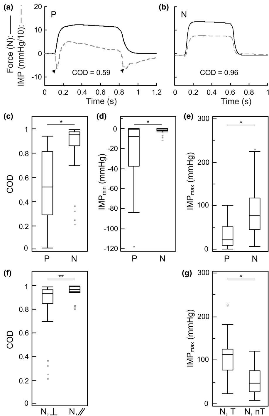
FIGURE 3. Representative force (solid black) and intramuscular pressure (IMP; dashed grey) measured using a sensor with a (a) polyimide (P) housing and a (b) nitinol (N) housing during isometric activation of a rabbit tibialis anterior at optimal length. Black arrowheads indicate negative pressure artifacts. Box plots showing the (c) coefficient of determination (COD) between force and IMP, (d) minimum IMP ( IMP_{min} ) and (e) maximum IMP ( IMP_{max} ) measured using four polyimide housing sensors ( n = 46 trials) and seven nitinol housing sensors ( n = 47 trials). Sub-analyses of nitinol housing sensor on the effect of (f) insertion direction relative to fiber shortening direction (perpendicular, \perp , n = 31 trials; parallel, \parallel , n = 16 trials) on the COD and (g) the presence (tissue, T; n = 23 trials) or absence (no tissue, nT, n = 24 trials) of tissue accumulation in the recess on the IMP_{max} . Sensors with nitinol housings had a superior force-IMP correlation compared to polyimide housings and eliminated negative pressure artifacts. Parallel insertion resulted in a significantly greater COD compared to perpendicular insertion. The presence of tissue resulted in a significantly greater IMP_{max} compared to when tissue was not present in the recess. * p < 0.001 , ** p < 0.05 .
